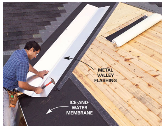
The installation of flashing in the new valley is shown. Note that existing shingles have been removed and ice and water barrier has been applied.
